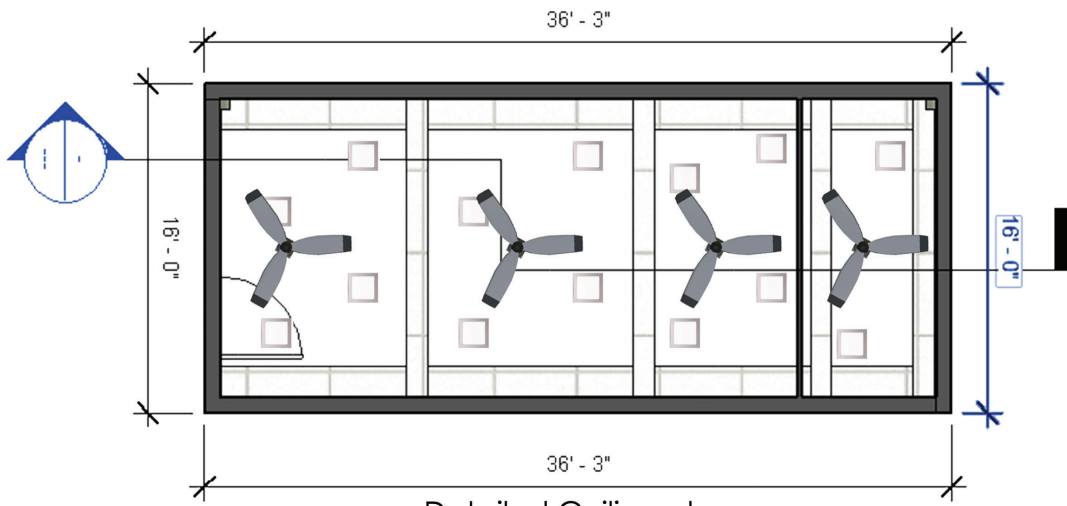
Detailed Ceiling plan
