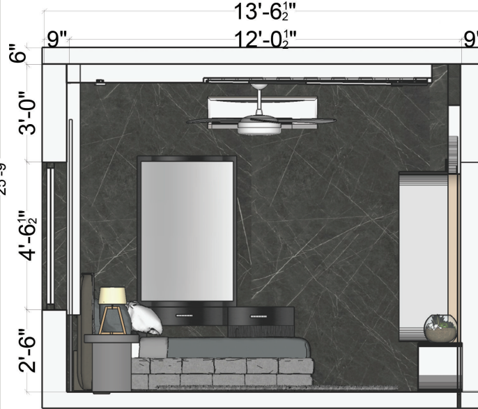
Interior Elevation A
