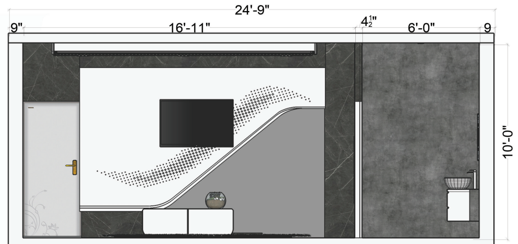
Interior Elevation D
