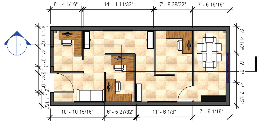
Detailed Floor plan
