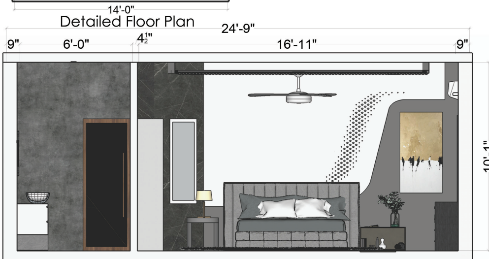
Interior Elevation C
