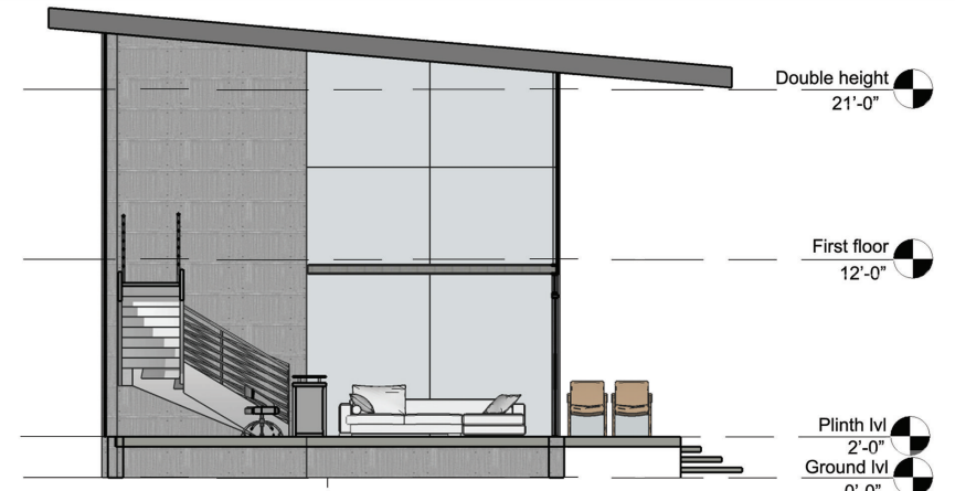
Section A
